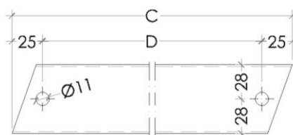
Alzado diagonal
